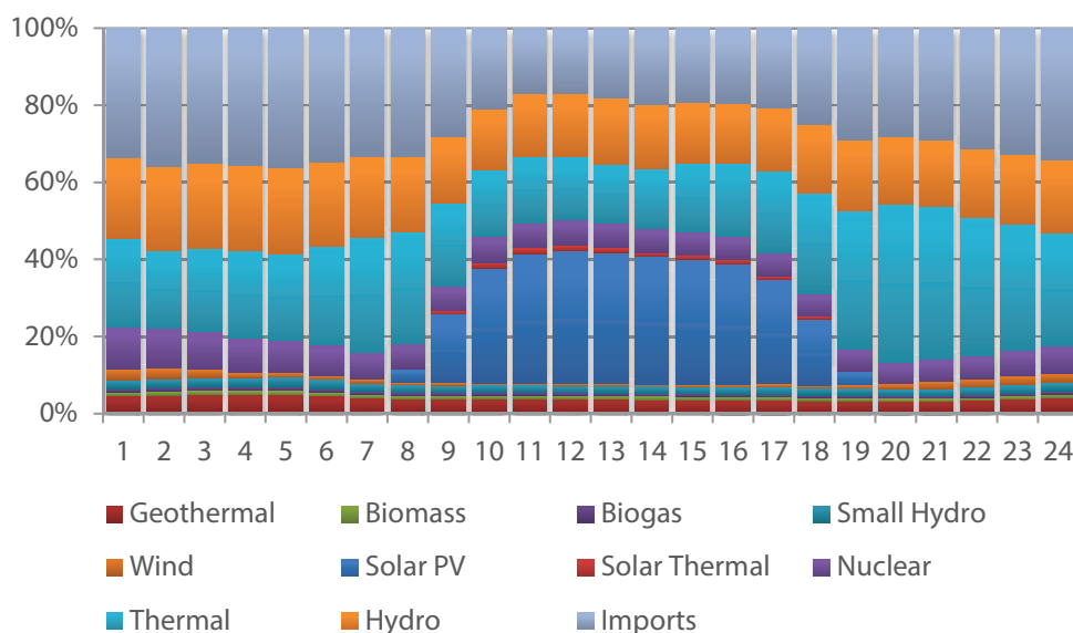
Figure 4: CAISO Hourly Production by Resource Type for 3/13/2017
