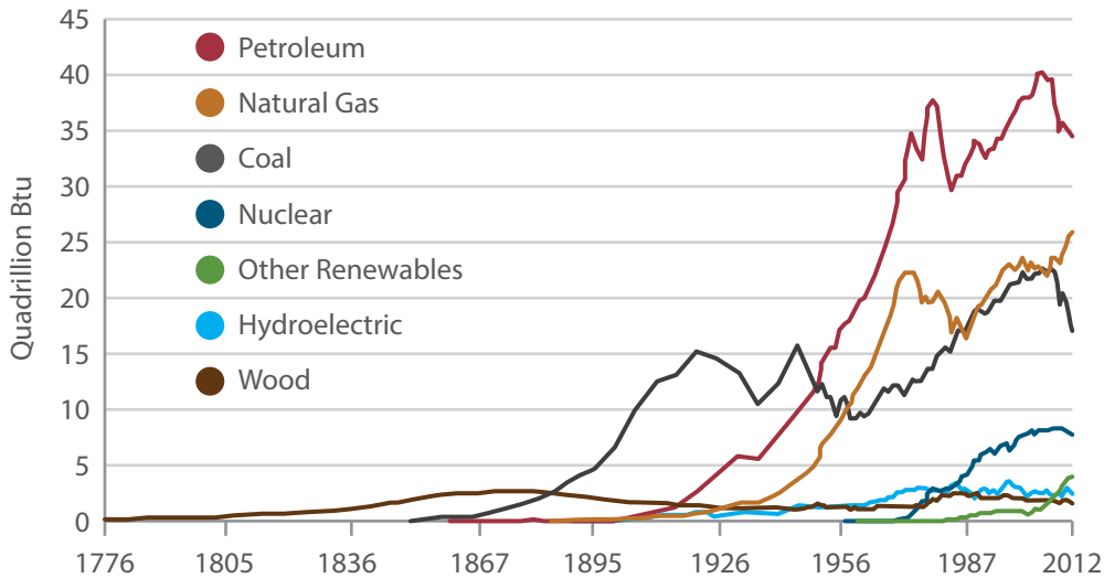
Figure 1: History of Energy Consumption in the United States (1776-2012)
